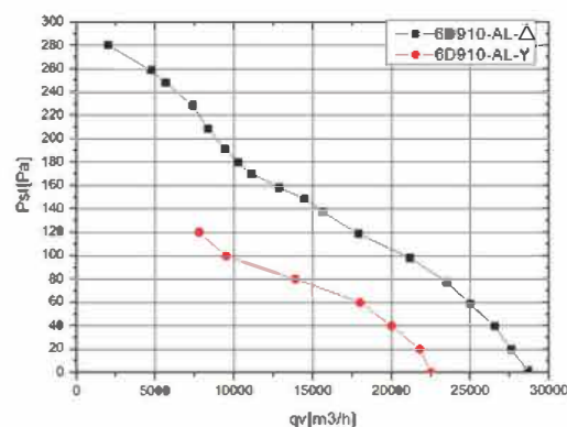
FLOW RATE CURVE :
