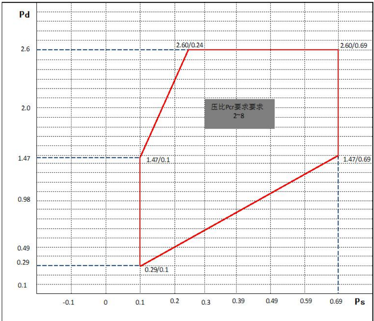
压缩机运行范围 Operation Limitation of Compressor 单位MPa (表压) Unit : MPa (G)
